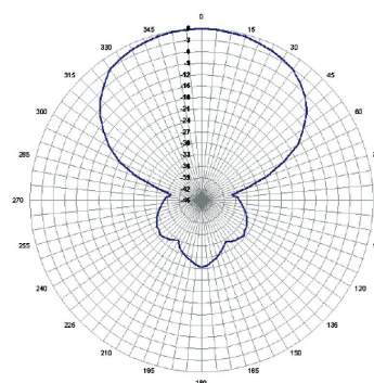
Horizontal plane 2400 MHz
