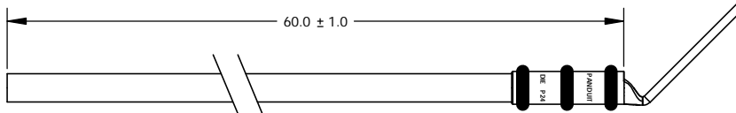
FACTORY CRIMPED #6 AWG/16mm SQ. COMMON BONDING NETWORK (CBN) JUMPER WIRE ASSEMBLY (QTY. 1) INCLUDES: LCC6-14JAWH (QTY. 1) #6 AWG/16mm SQ. WIRE - GREEN/YELLOW INSULATION 60" LONG
