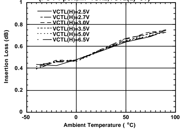
Insertion Loss vs. Ambient Temperature (PC-P1 port, f_{in}=1GHz, V_{CTL(L)}=0V )
