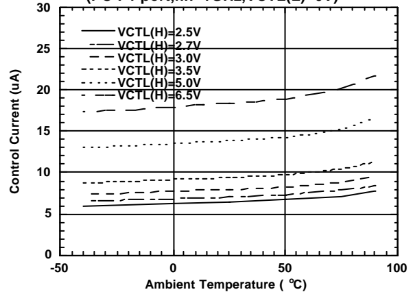
ICTL vs. Ambient Temperature (PC-P1 port, f_{in}=1GHz, V_{CTL(L)}=0V )
