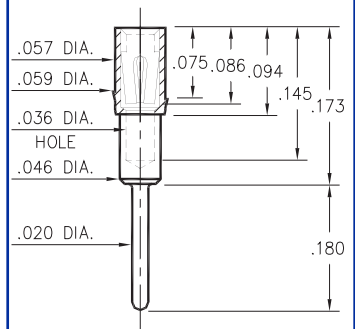
1753-0-15-XX-30-XX-04-0 Press-fit in .057 mounting hole
