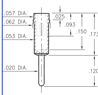
0307-0-15-XX-30-XX-04-0 Press-fit in .059 mounting hole
