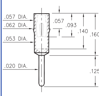
0240-0-15-XX-30-XX-04-0 Press-fit in .059 mounting hole
