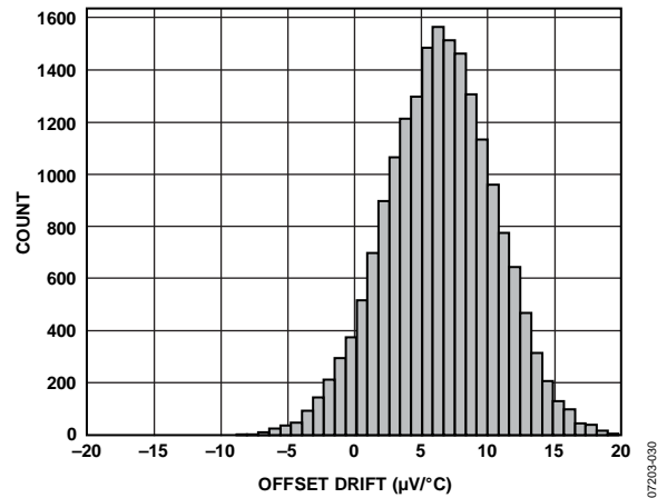
Figure 25. Offset Drift
