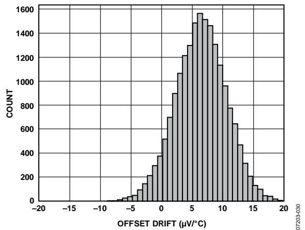
Figure 25. Offset Drift
