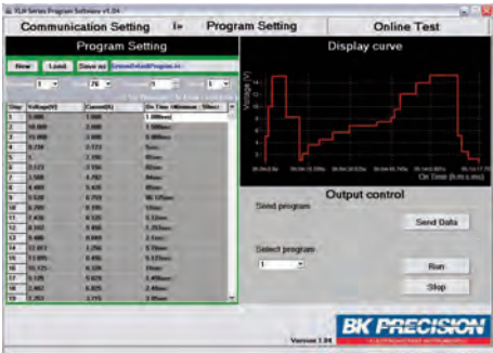
Create, save & load program lists. View output characteristic curves and export data to a file.
