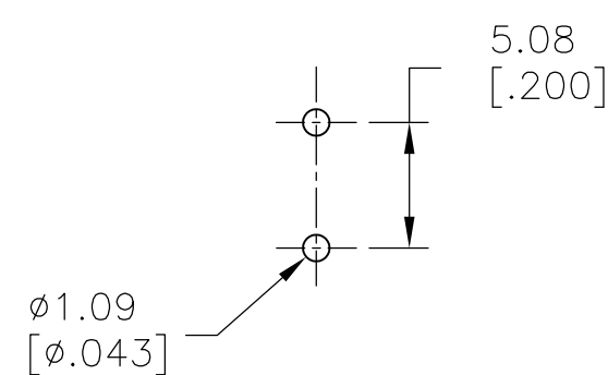
P.C. MOUNTING
