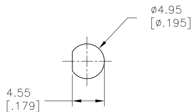
PANEL MOUNTING
