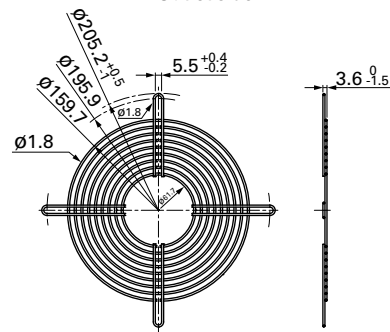
Outlet side
