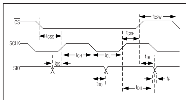
Figure 4. Detailed Serial Interface Timing Diagram
