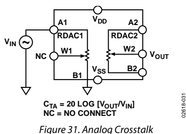
Figure 31. Analog Crosstalk
