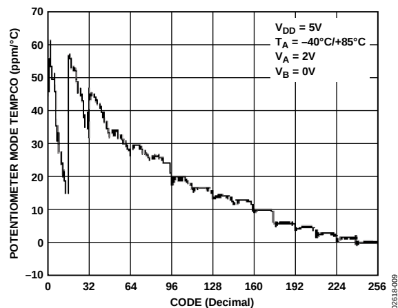
Figure 9. \Delta V_{WB}/\Delta T vs. Code; R_{AB} = 10\text{ k}\Omega , V_{DD} = 5V
