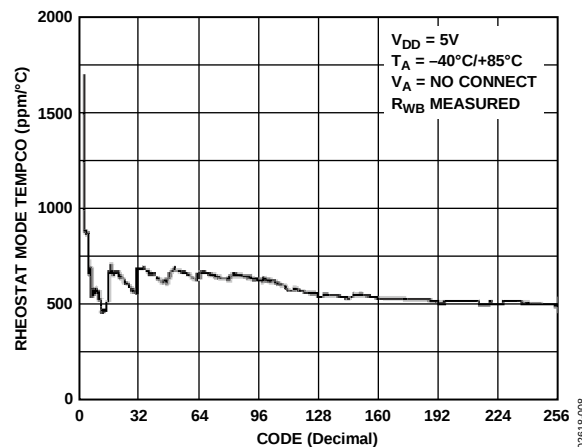
Figure 8. \Delta R_{WB}/\Delta T vs. Code; R_{AB} = 10\text{ k}\Omega , V_{DD} = 5V
