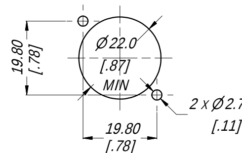
PANEL CUT OUT 1:1 (CONNECTOR FRONT VIEW)
