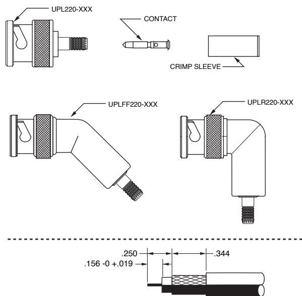
CABLE STRIPPING DIMENSIONS (SHOWN AS ACTUAL SIZE: USE AS STRIPPING TEMPLATE)
