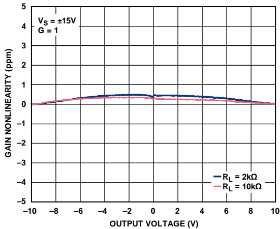
Figure 36. Gain Nonlinearity (G = 1)
