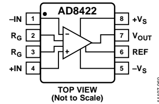
Figure 57. Pinout Diagram
