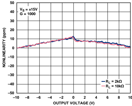
Figure 39. Gain Nonlinearity (G = 1000)
