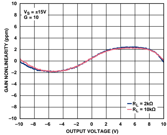
Figure 37. Gain Nonlinearity (G = 10)
