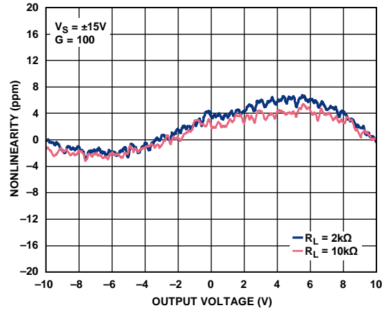
Figure 38. Gain Nonlinearity (G = 100)
