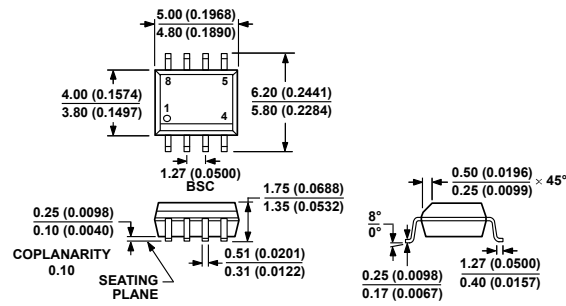
Figure 65. 8-Lead Standard Small Outline Package [SOIC_N] Narrow Body (R-8)
