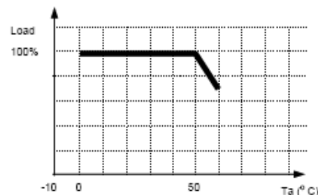
DERATING CURVE
