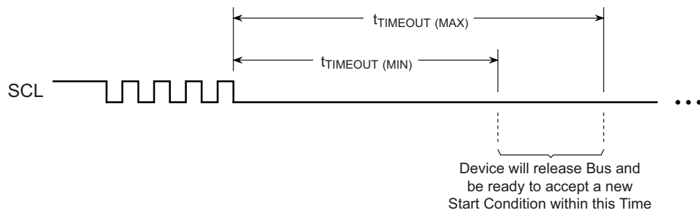
Figure 10-2. SMBus Timeout
