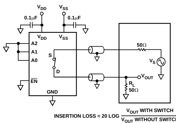
Figure 30. Bandwidth
