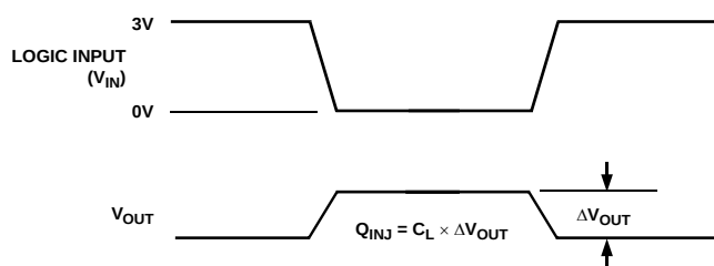
Figure 28. Charge Injection
