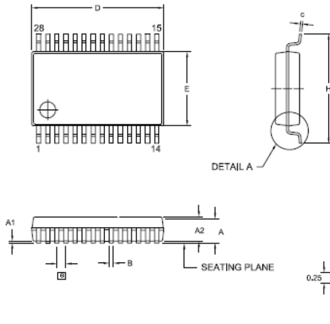
Figure 9 - 28-Pin Small Shrink Outline Package (SSOP)
