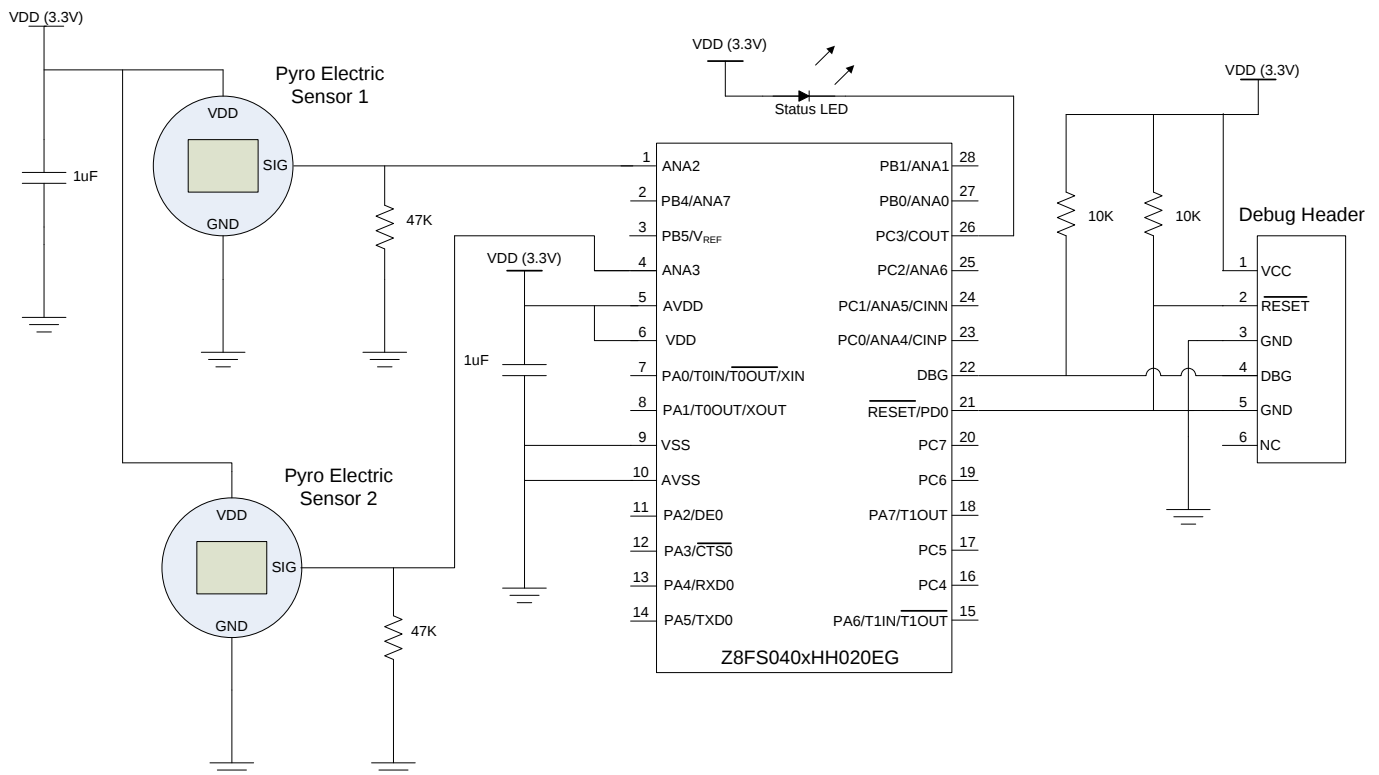
Figure 14 - Required Circuit Connections for Z8FS040xHJ20EG (28 Pin) Motion Detection MCU – Dual Pyro Mode
