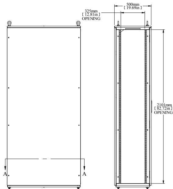
L.S. VIEW
