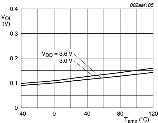
Fig 27. SDA output V_{OL} at I_{OL} = 3.0\text{ mA}
