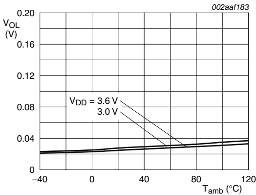
Fig 25. SDA output V_{OL} at I_{OL} = 0.7\text{ mA}
