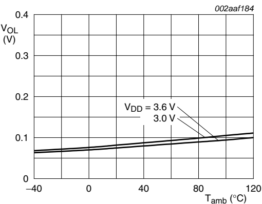
Fig 26. SDA output V_{OL} at I_{OL} = 2.1\text{ mA}
