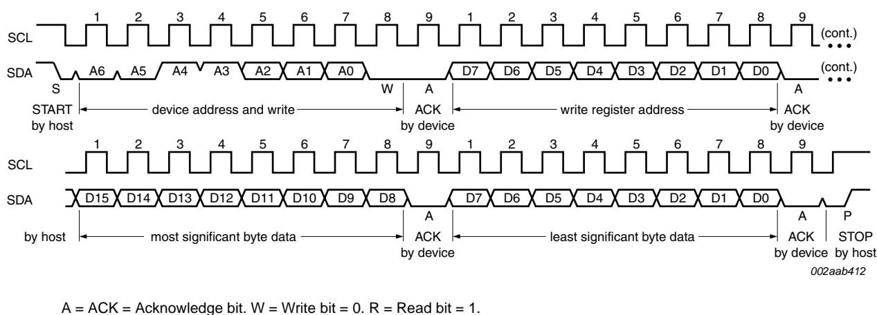
Fig 7. SMBus/I 2 C-bus write to the Pointer register followed by a write data word
