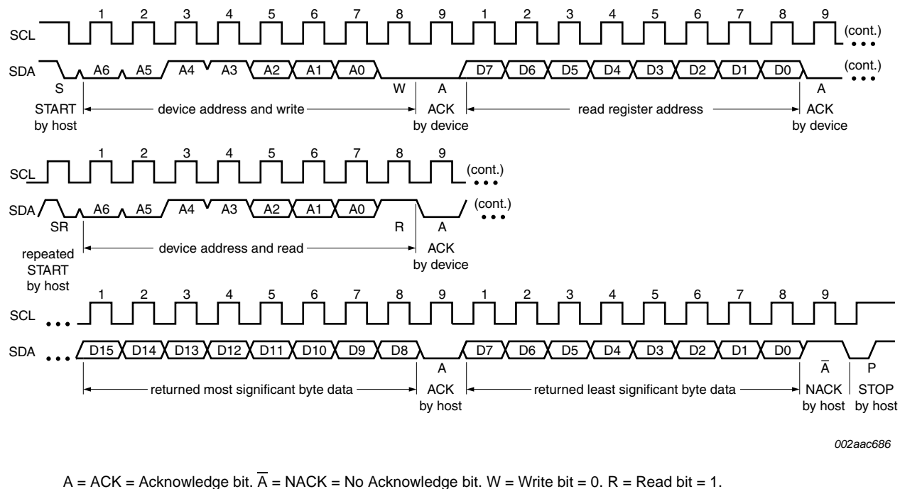
Fig 8. SMBus/I 2 C-bus write to Pointer register followed by a repeated START and an immediate data word read
