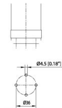
Direct Mounting
