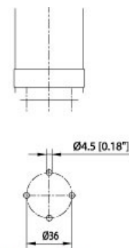
Direct Mounting
