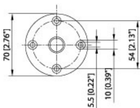
Tubular Stand/Plinth
