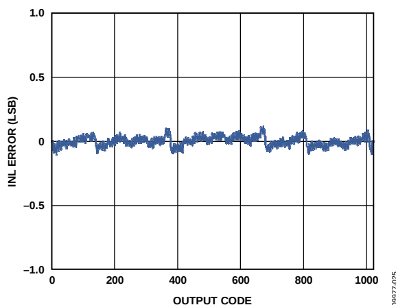
Figure 33. INL Error with f_{IN} = 9.7 MHz
