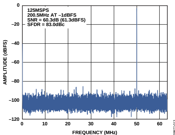
Figure 13. Single-Tone FFT with f_{IN} = 200.5 MHz
