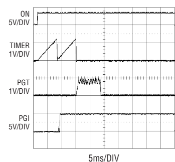
Power-Up Waveforms
