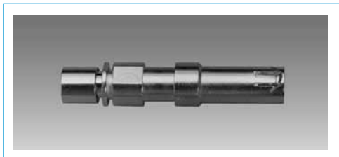
Coax Contact, Socket for use in MS/Standard MIL-DTL-5015 and Heavy Duty MIL-DTL-22992 Connectors
