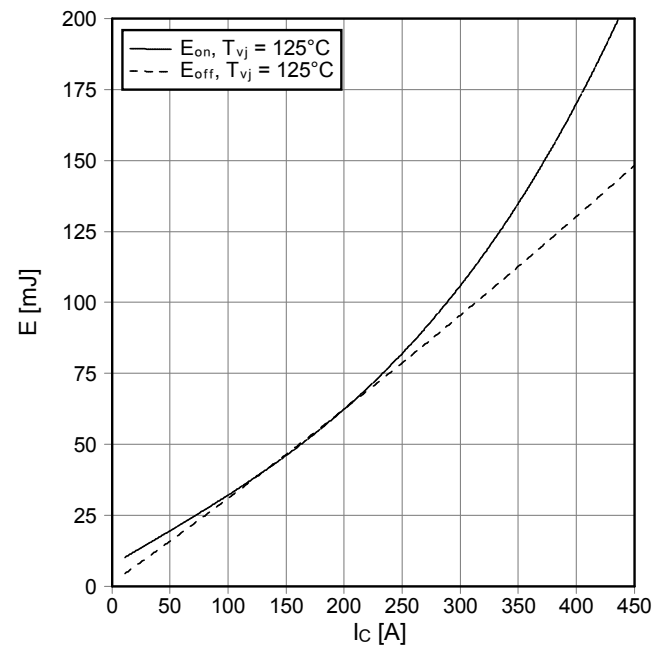
Schaltverluste IGBT-Wechselr. (typisch) switching losses IGBT-inverter (typical) E_{on} = f(I_c) , E_{off} = f(I_c) V_{GE} = \pm 15\text{ V} , R_{Gon} = 6.2\ \Omega , R_{Goff} = 6.2\ \Omega , V_{CE} = 900\text{ V}
