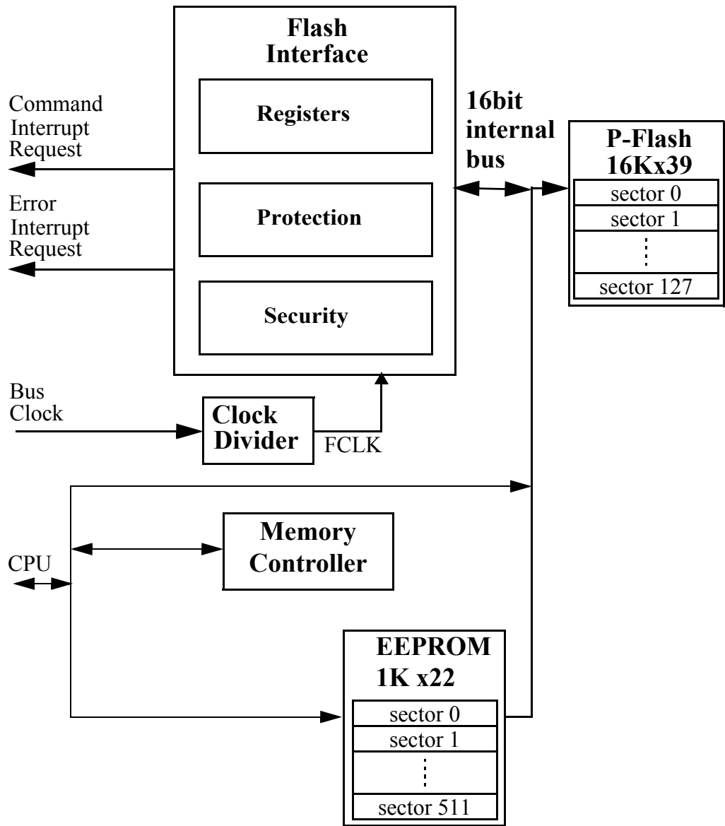
Figure 21-1. FTMZ64K2K Block Diagram
