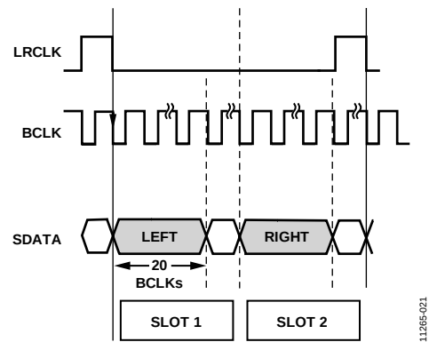
Figure 21. TDM2 Channel 1 and Channel 2, CONFIG Pin Tied to GND
