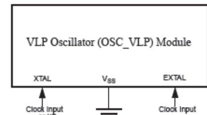
Configuration for external clock
