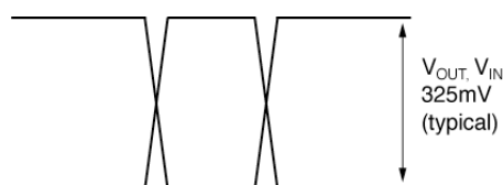
Figure 2c. Single-Ended Swing
