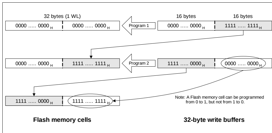
Figure 11 D-Flash Programming
