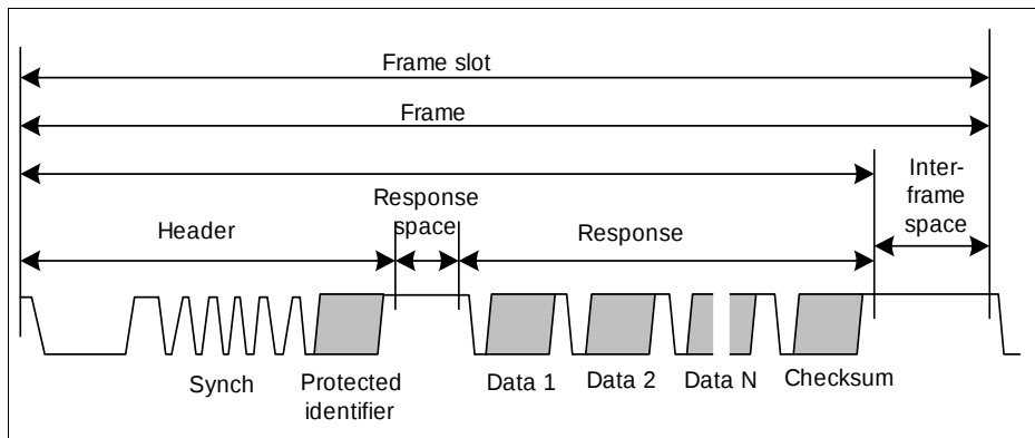
Figure 29 Structure of LIN Frame
