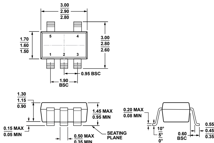
Figure 41. 5-Lead Small Outline Transistor Package [SOT-23] (RJ-5) Dimensions shown in millimeters
