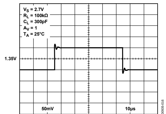
Figure 16. Small Signal Transient Response
