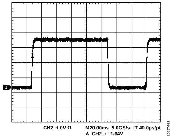
Figure 22. SYNC_OUT ( f_{\text{SYSCLK}}/384 )
