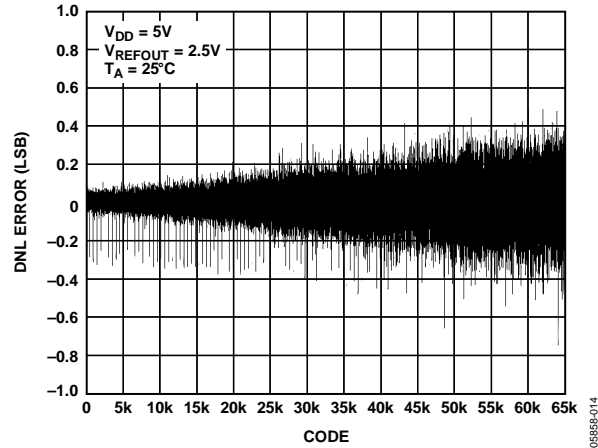
Figure 13. DNL—AD5663R-5
