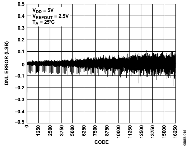
Figure 14. DNL—AD5643R-5
