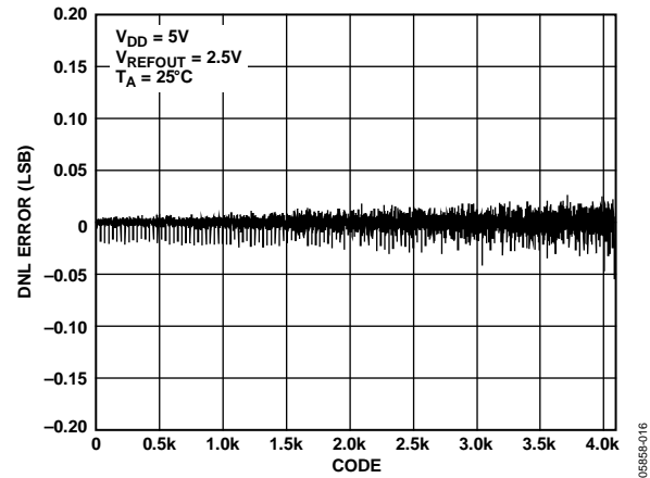
Figure 15. DNL—AD5623R-5
