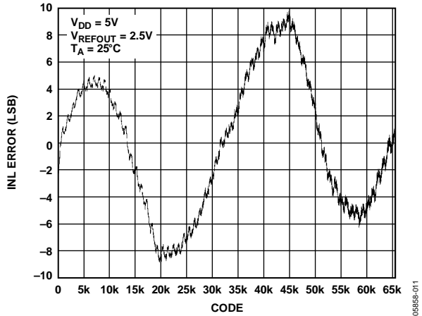
Figure 10. INL—AD5663R-5
