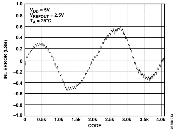
Figure 12. INL—AD5623R-5
