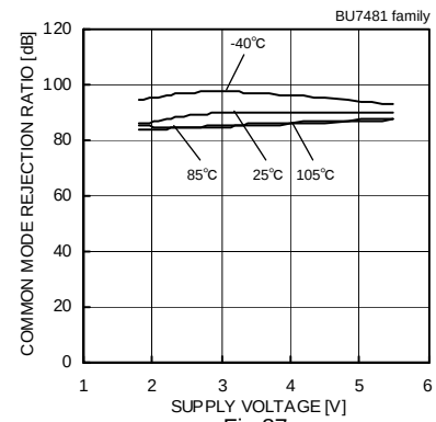
Fig.87 Common Mode Rejection Ratio – Supply Voltage (V DD =3[V])
