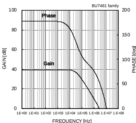
Fig.92 Voltage Gain—Frequency
