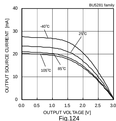
Fig.124 Output Source Current – Output Voltage (VDD=3[V])
