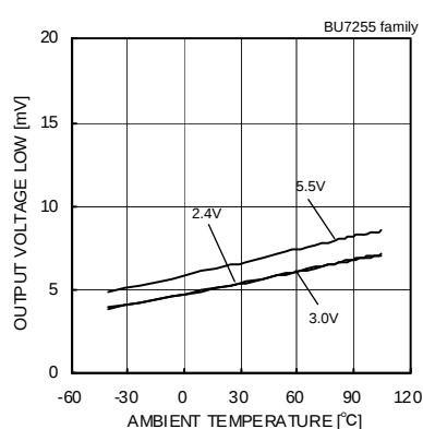
Fig.31 Output Voltage Low – Ambient Temperature (RL=10[kΩ])
