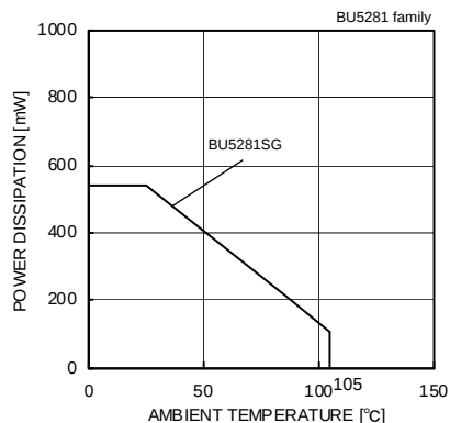
Fig.117 Derating curve
