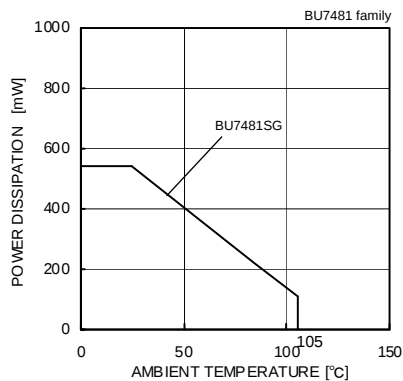
Fig.71 Derating curve
