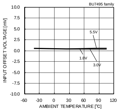
Fig.60 Input Offset Voltage – Ambient Temperature ( V_{icm}=V_{DD} , V_{OUT}=1.5[V] )
