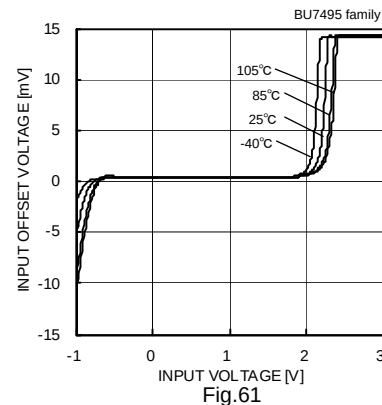
Fig.61 Input Offset Voltage – Input Voltage ( V_{DD}=3[V] )
