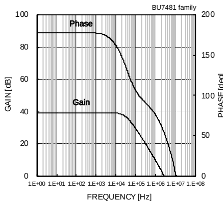
Fig.92 Voltage Gain—Frequency
