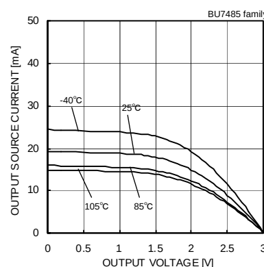
Fig.101 Output Source Current – Output Voltage (VDD=3[V])
