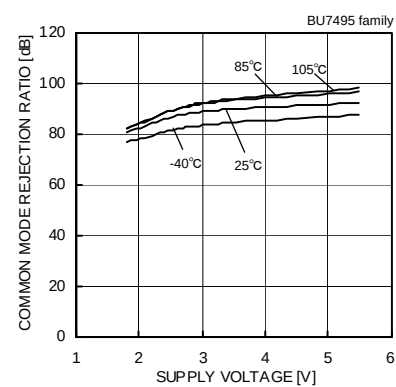
Fig.64 Common Mode Rejection Ratio – Supply Voltage ( V_{DD}=3[V] )
