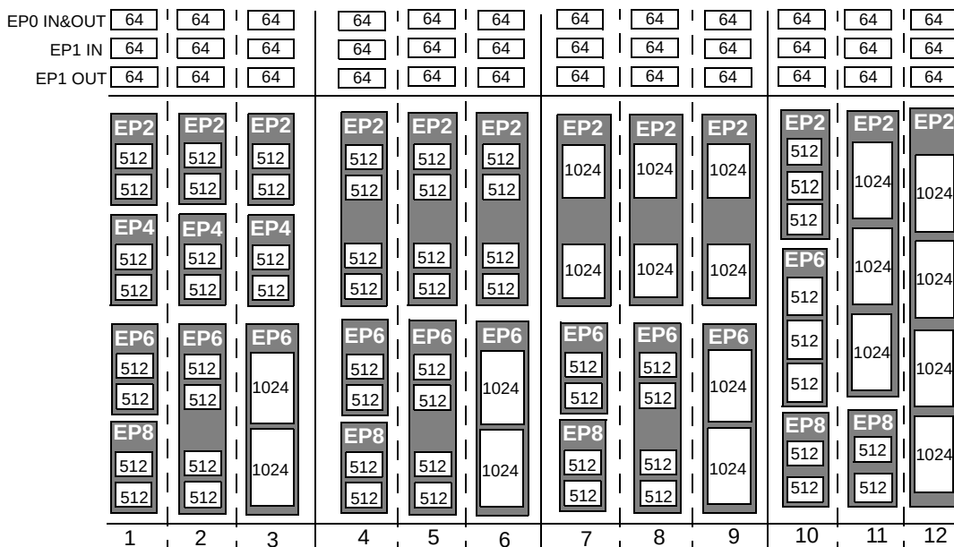
Figure 5. Endpoint Configuration
