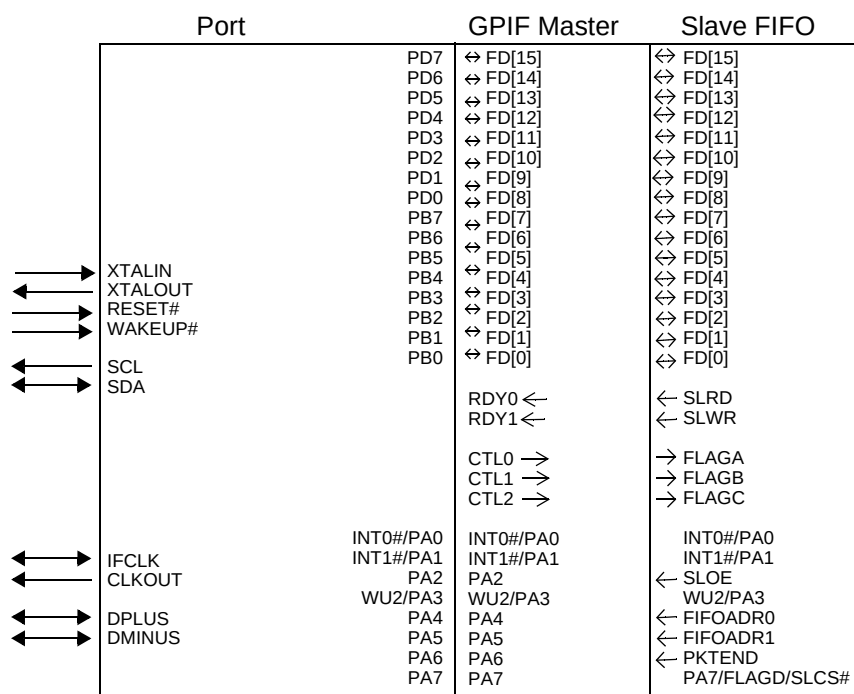
Figure 6. Signals
