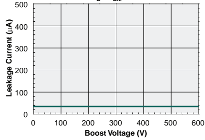
High/Middle Supply Leakage Current vs. V_B / V_{BM} Voltage
