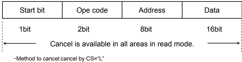
Fig.29 READ cancel available timing
