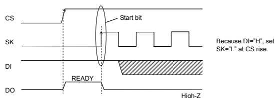
Fig.45 Start bit input timing at DI, DO direct connection
