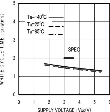
Fig.22 Write cycle time t_{E/W}
