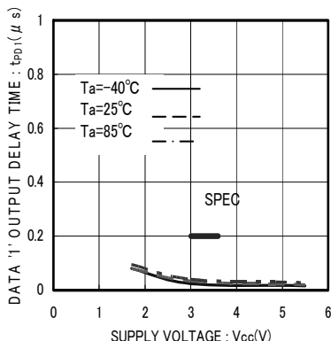
Fig.19 Data '1' output delay time t_{PD1}
