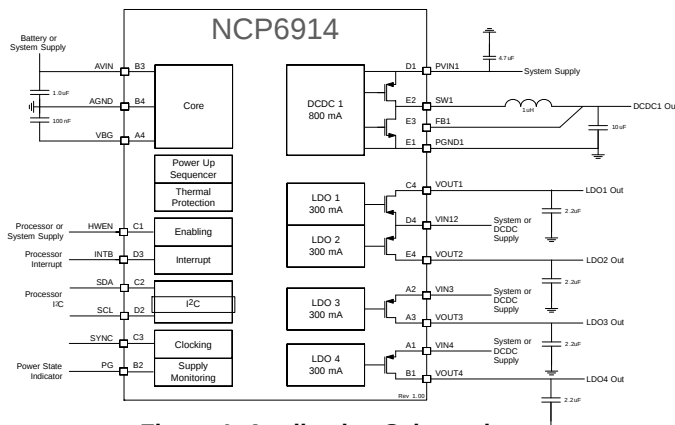
Figure 1. Application Schematic
